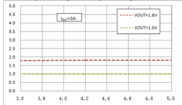
Input Voltage vs. Output Voltage
